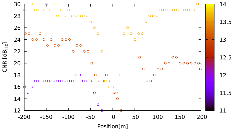
CNR vs position for G32 (L5) on HuaweiP40 - DOY 263 jam. 1
