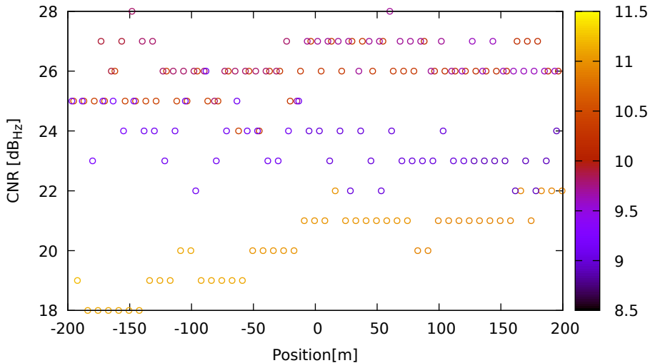
CNR vs position for G32 (L5) on HuaweiP40 - DOY 263 jam. 2
