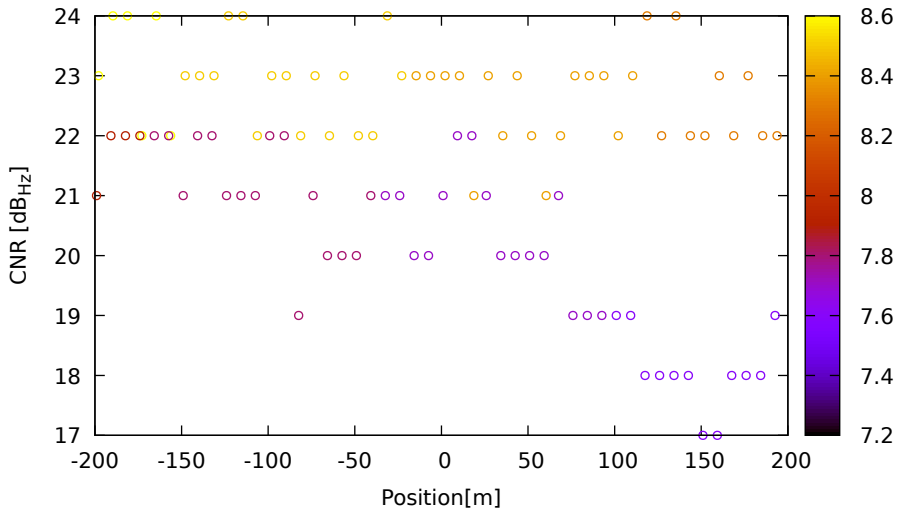
CNR vs position for G32 (L5) on HuaweiP40 - DOY 263 jam. 3
