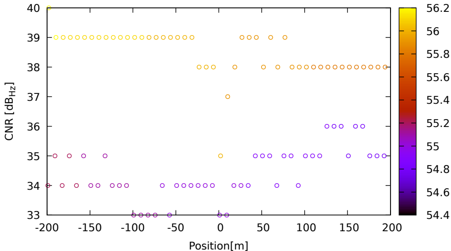
CNR vs position for R01 (G1) on HuaweiP40 - DOY 263 jam. 3
