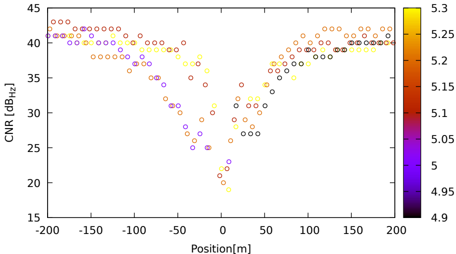
CNR vs position for R09 (G1) on HuaweiP40 - DOY 263 jam. 1
