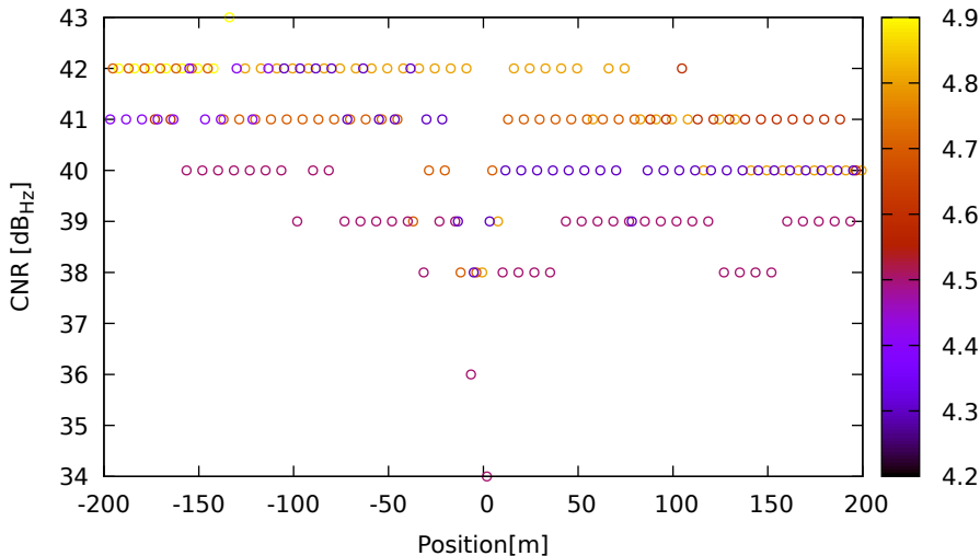
CNR vs position for R09 (G1) on HuaweiP40 - DOY 263 jam. 2
