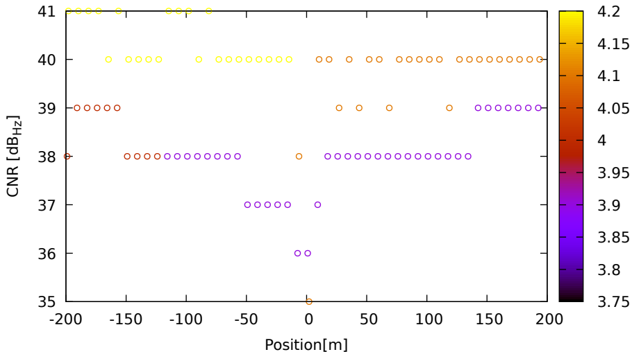
CNR vs position for R09 (G1) on HuaweiP40 - DOY 263 jam. 3
