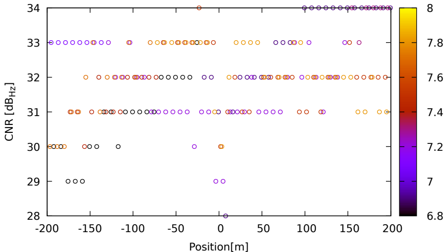
CNR vs position for R10 (G1) on HuaweiP40 - DOY 263 jam. 2
