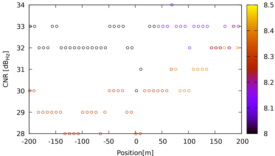
CNR vs position for R10 (G1) on HuaweiP40 - DOY 263 jam. 3
