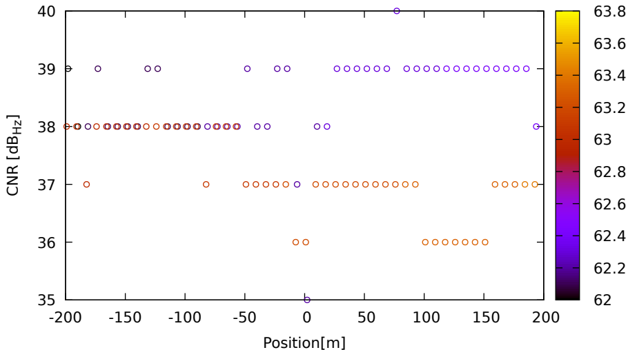
CNR vs position for R17 (G1) on HuaweiP40 - DOY 263 jam. 3
