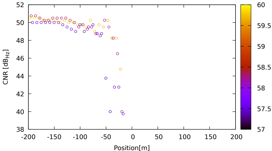
CNR vs position for C11 (B1) on LeicaGS18 - DOY 263 jam. 2
