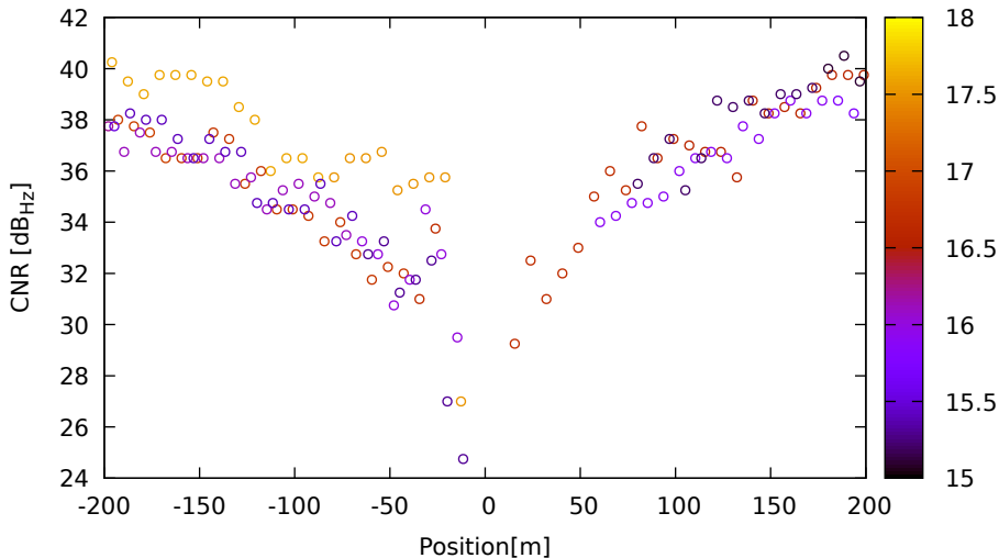
CNR vs position for C12 (B1) on LeicaGS18 - DOY 263 jam. 1
