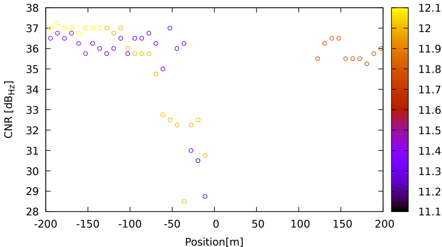
CNR vs position for C12 (B1) on LeicaGS18 - DOY 263 jam. 3
