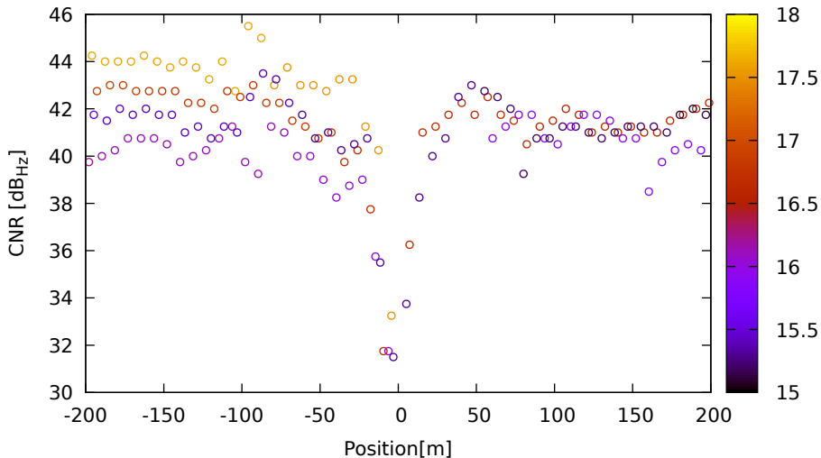
CNR vs position for C12 (B3) on LeicaGS18 - DOY 263 jam. 1
