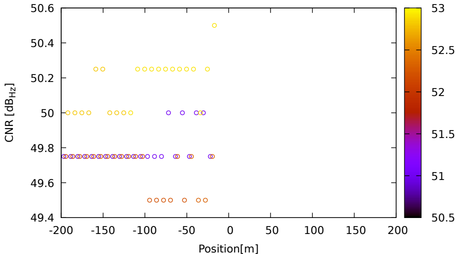
CNR vs position for C14 (B3) on LeicaGS18 - DOY 263 jam. 2
