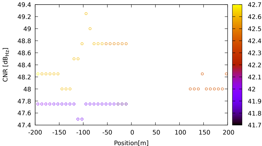
CNR vs position for C21 (B3) on LeicaGS18 - DOY 263 jam. 3
