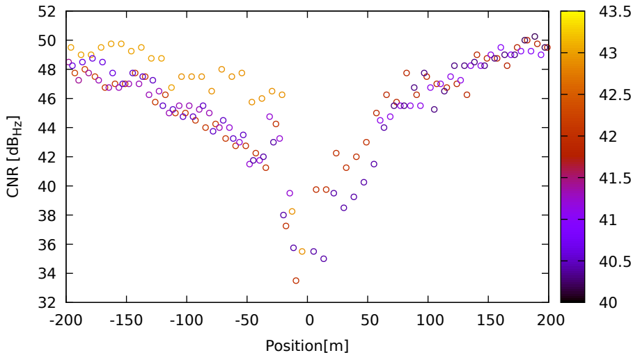
CNR vs position for C34 (B1) on LeicaGS18 - DOY 263 jam. 1
