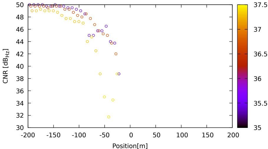
CNR vs position for E04 (E1) on LeicaGS18 - DOY 263 jam. 2
