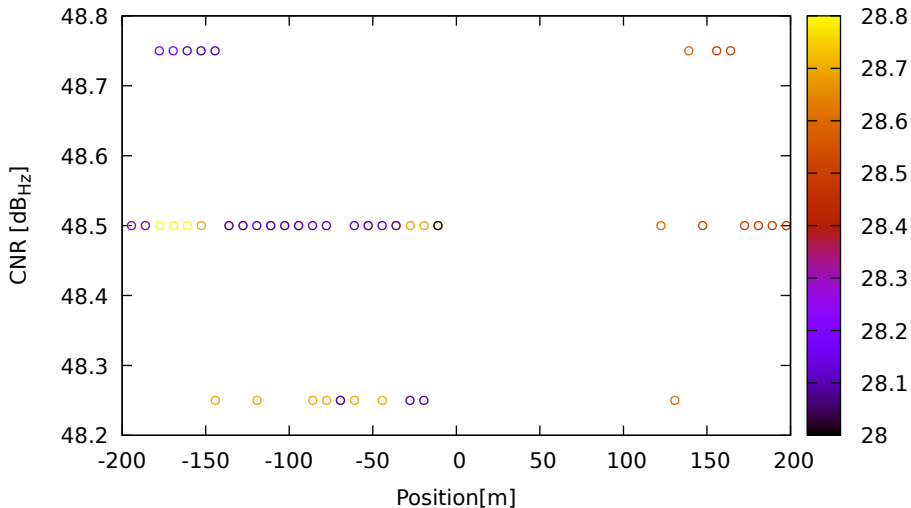
CNR vs position for E33 (E5a) on LeicaGS18 - DOY 263 jam. 3
