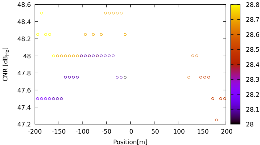
CNR vs position for E33 (E5b) on LeicaGS18 - DOY 263 jam. 3
