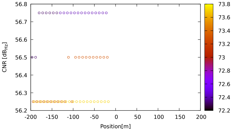
CNR vs position for G03 (L5) on LeicaGS18 - DOY 263 jam. 2
