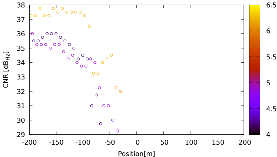
CNR vs position for G08 (L1) on LeicaGS18 - DOY 263 jam. 2
