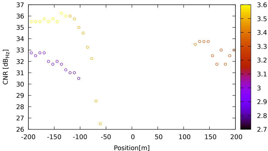
CNR vs position for G08 (L1) on LeicaGS18 - DOY 263 jam. 3
