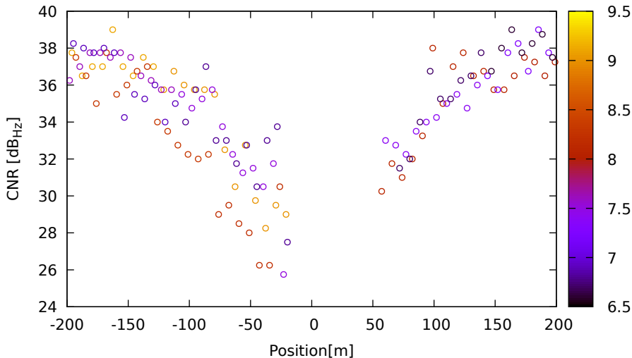
CNR vs position for G08 (L2) on LeicaGS18 - DOY 263 jam. 1
