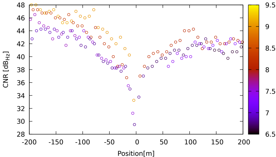
CNR vs position for G08 (L5) on LeicaGS18 - DOY 263 jam. 1
