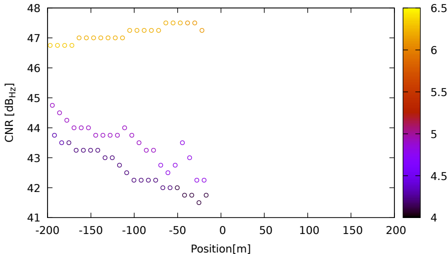
CNR vs position for G08 (L5) on LeicaGS18 - DOY 263 jam. 2
