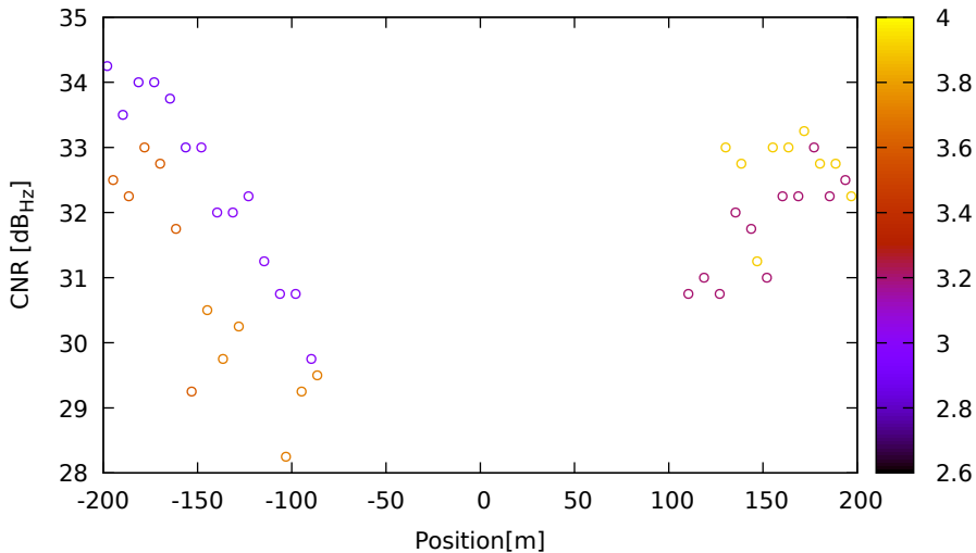
CNR vs position for G09 (L1) on LeicaGS18 - DOY 263 jam. 1
