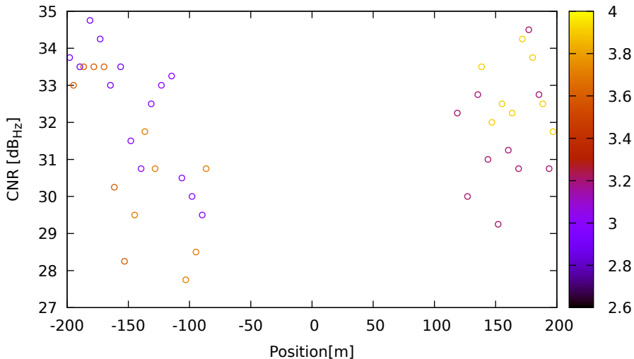
CNR vs position for G09 (L2) on LeicaGS18 - DOY 263 jam. 1
