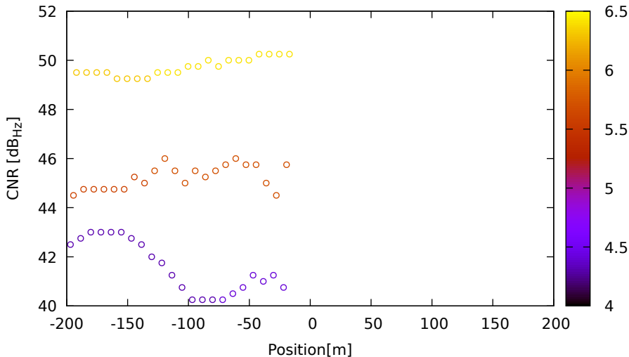
CNR vs position for G09 (L5) on LeicaGS18 - DOY 263 jam. 2
