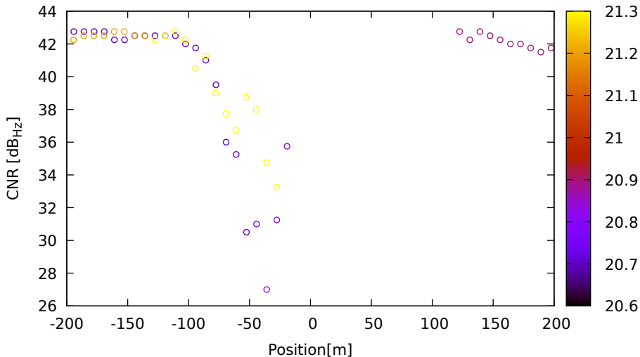
CNR vs position for G19 (L1) on LeicaGS18 - DOY 263 jam. 3
