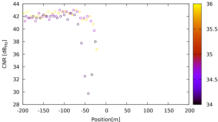
CNR vs position for G22 (L2) on LeicaGS18 - DOY 263 jam. 2
