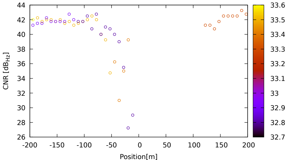
CNR vs position for G22 (L2) on LeicaGS18 - DOY 263 jam. 3
