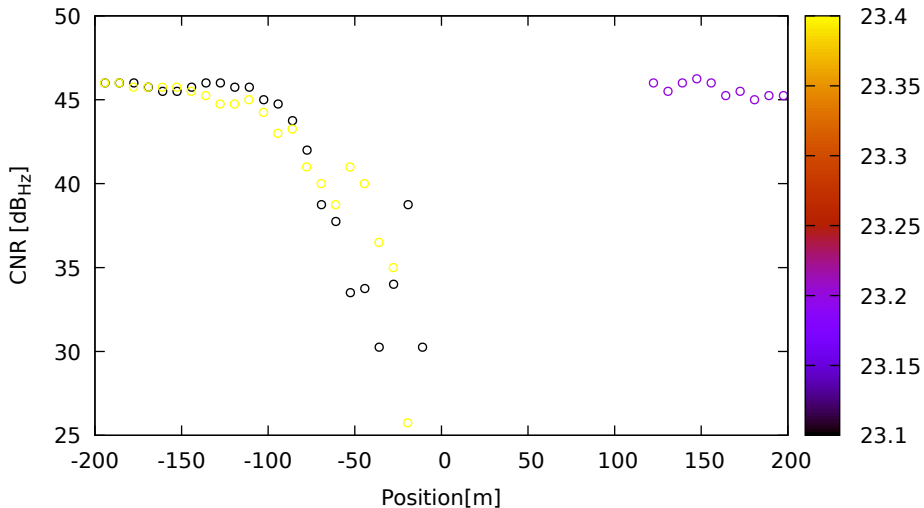
CNR vs position for G31 (L1) on LeicaGS18 - DOY 263 jam. 3
