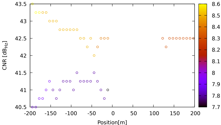
CNR vs position for G32 (L5) on LeicaGS18 - DOY 263 jam. 3
