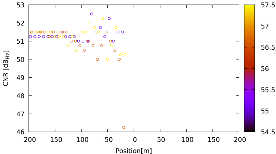
CNR vs position for R02 (G1) on LeicaGS18 - DOY 263 jam. 2
