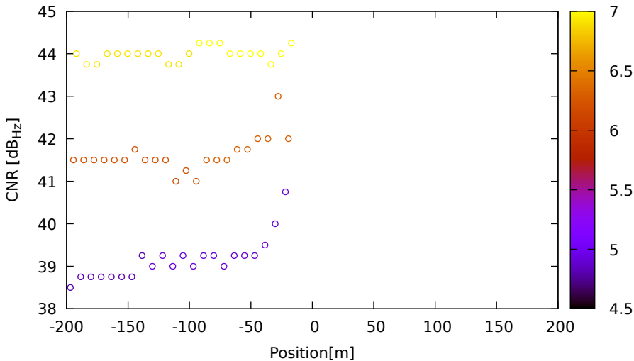
CNR vs position for R03 (G2) on LeicaGS18 - DOY 263 jam. 2
