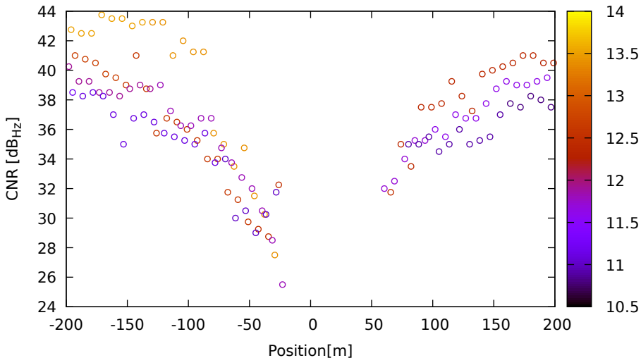
CNR vs position for R08 (G1) on LeicaGS18 - DOY 263 jam. 1
