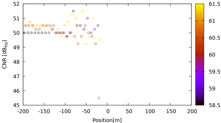
CNR vs position for R17 (G1) on LeicaGS18 - DOY 263 jam. 2
