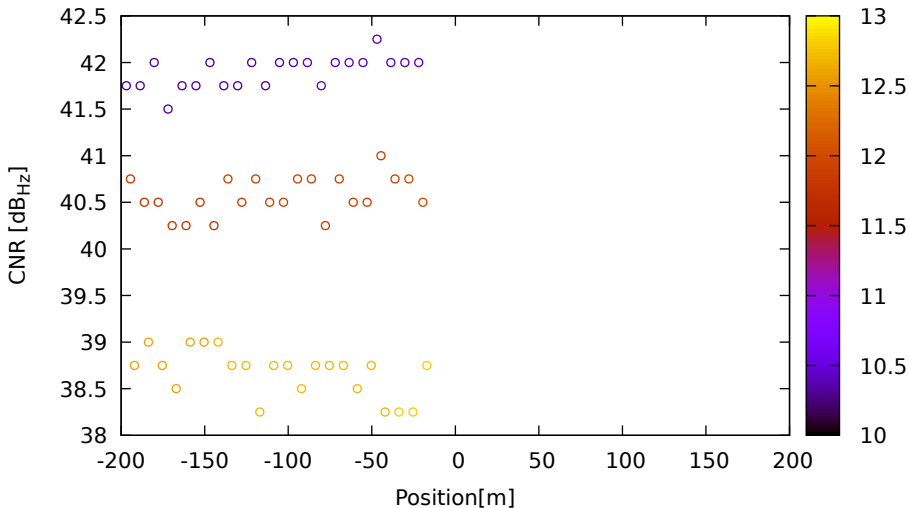
CNR vs position for R18 (G2) on LeicaGS18 - DOY 263 jam. 2
