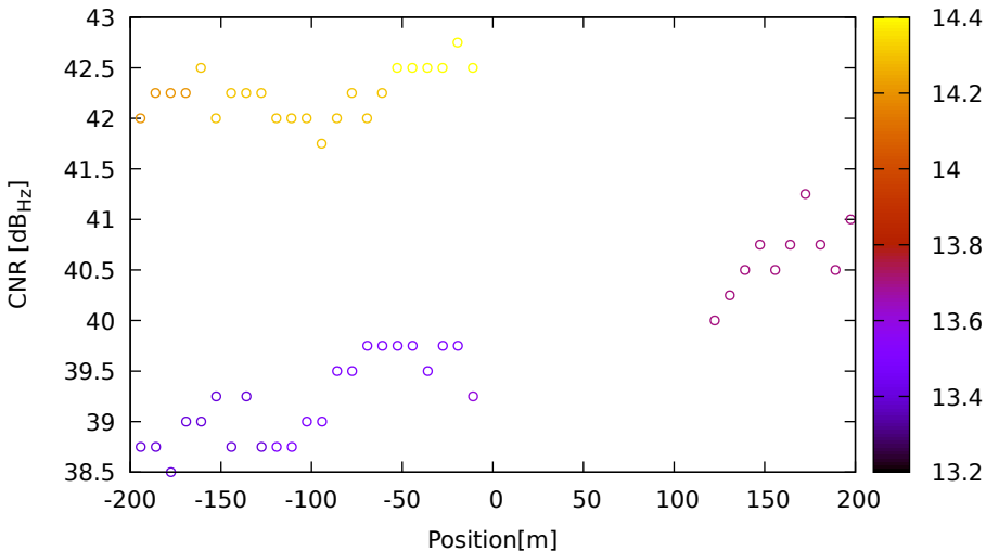
CNR vs position for R18 (G2) on LeicaGS18 - DOY 263 jam. 3
