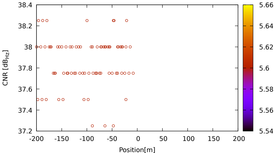
CNR vs position for C02 (B3) on LeicaGS18 - DOY 263 jam. 2
