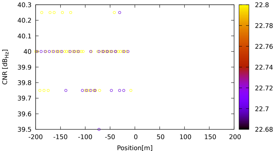
CNR vs position for C05 (B3) on LeicaGS18 - DOY 263 jam. 2
