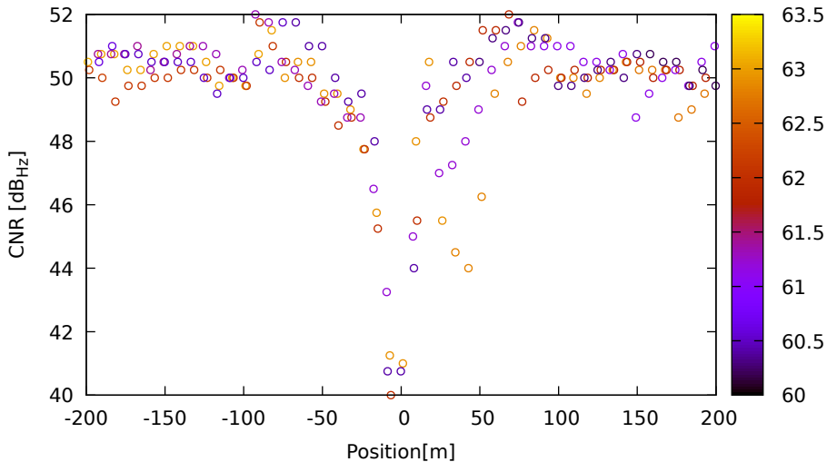
CNR vs position for C11 (B3) on LeicaGS18 - DOY 263 jam. 1
