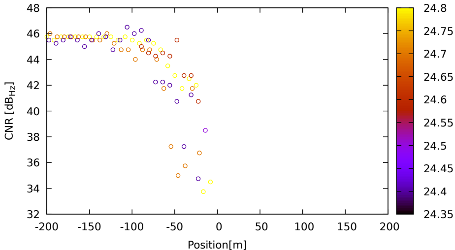
CNR vs position for C16 (B1) on LeicaGS18 - DOY 263 jam. 2
