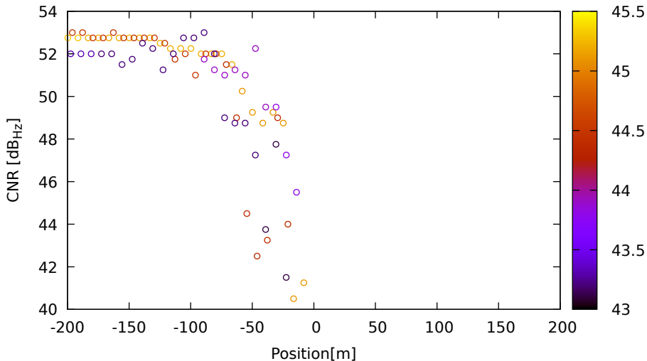
CNR vs position for C21 (B1) on LeicaGS18 - DOY 263 jam. 2
