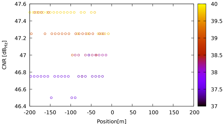
CNR vs position for C34 (B3) on LeicaGS18 - DOY 263 jam. 2
