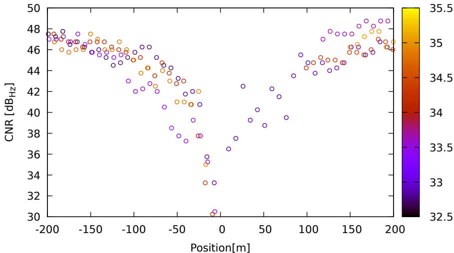
CNR vs position for E04 (E1) on LeicaGS18 - DOY 263 jam. 1
