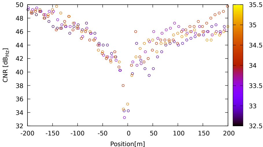
CNR vs position for E04 (E5a) on LeicaGS18 - DOY 263 jam. 1
