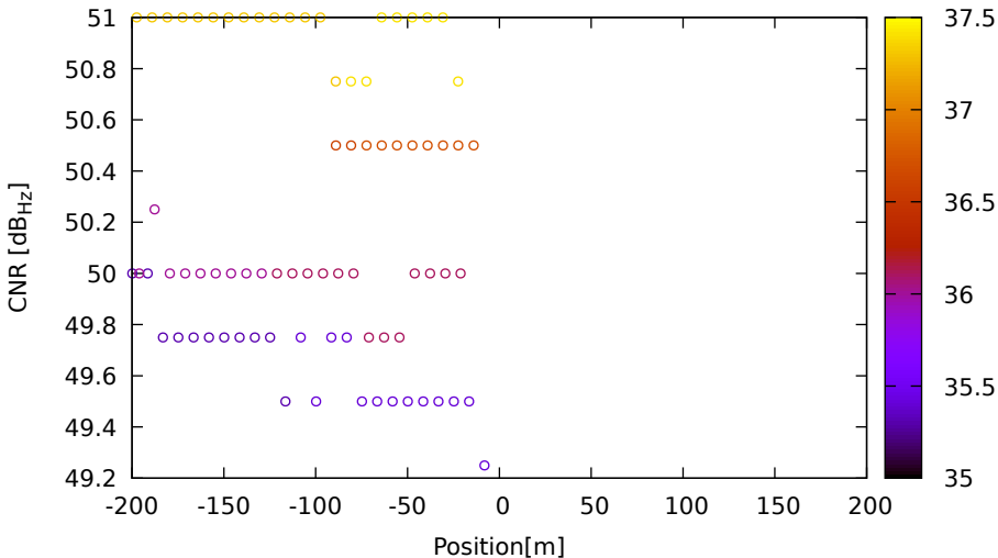
CNR vs position for E04 (E5b) on LeicaGS18 - DOY 263 jam. 2
