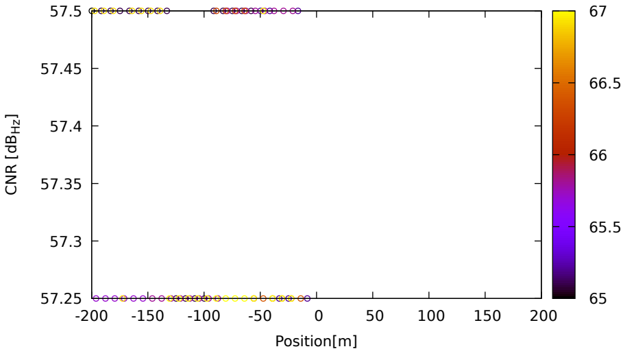
CNR vs position for E10 (E5) on LeicaGS18 - DOY 263 jam. 2
